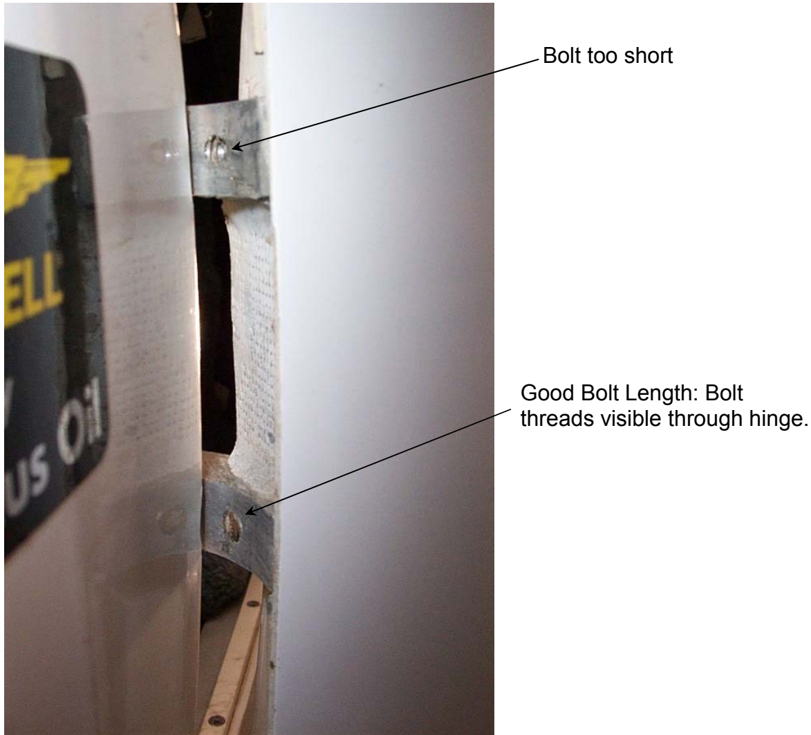
Figure 1. Hinge Bolt Detail
